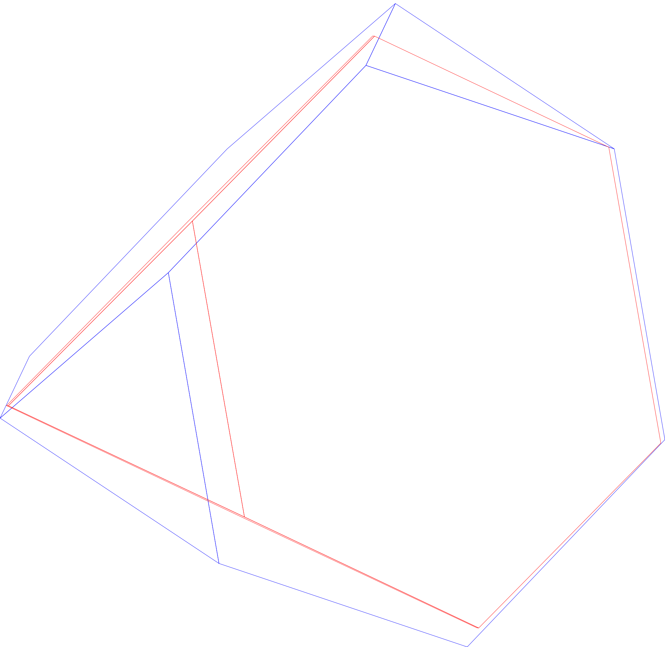
Truncated Tetrahedron
