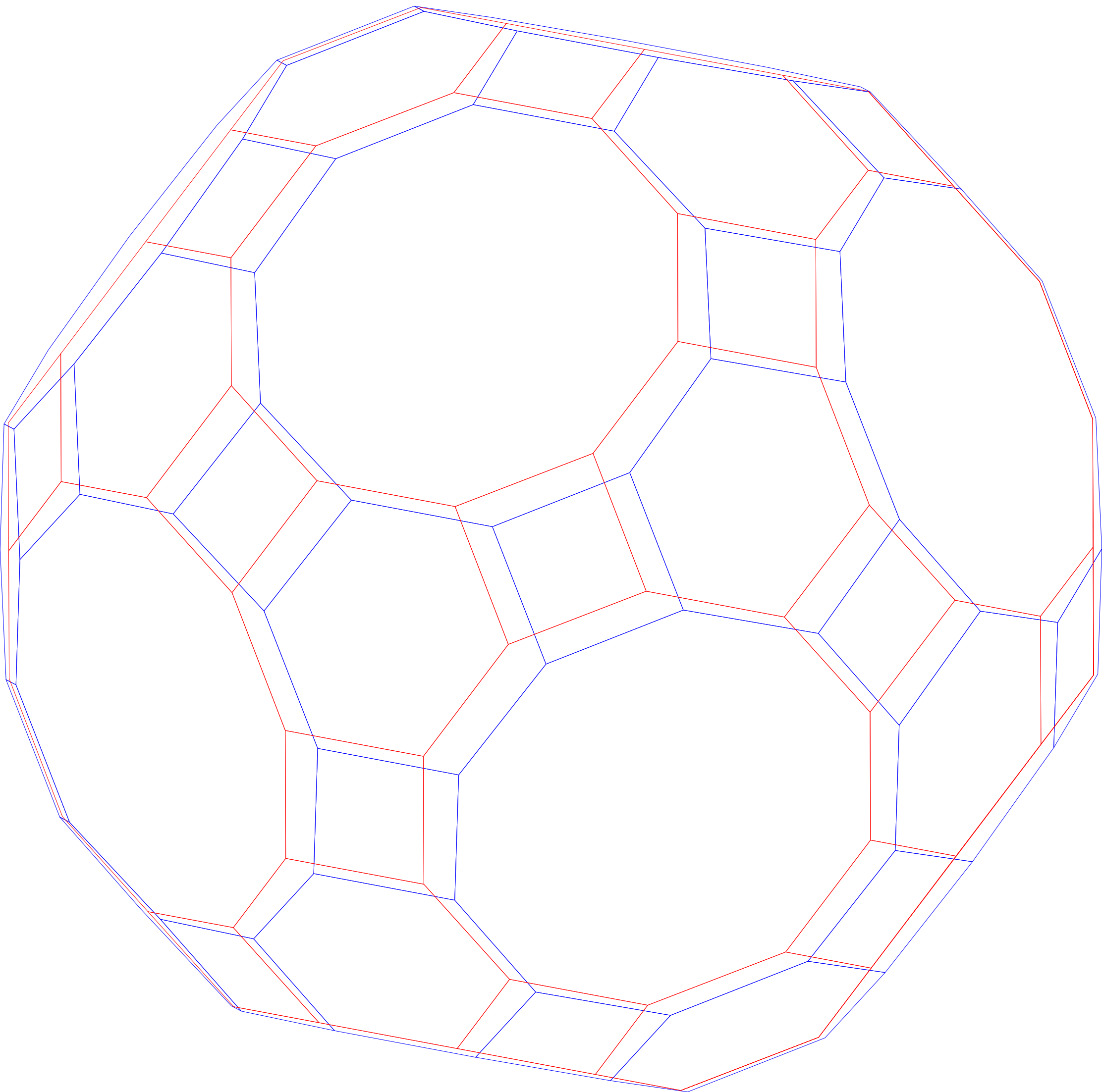
Truncated Icosidodecahedron
