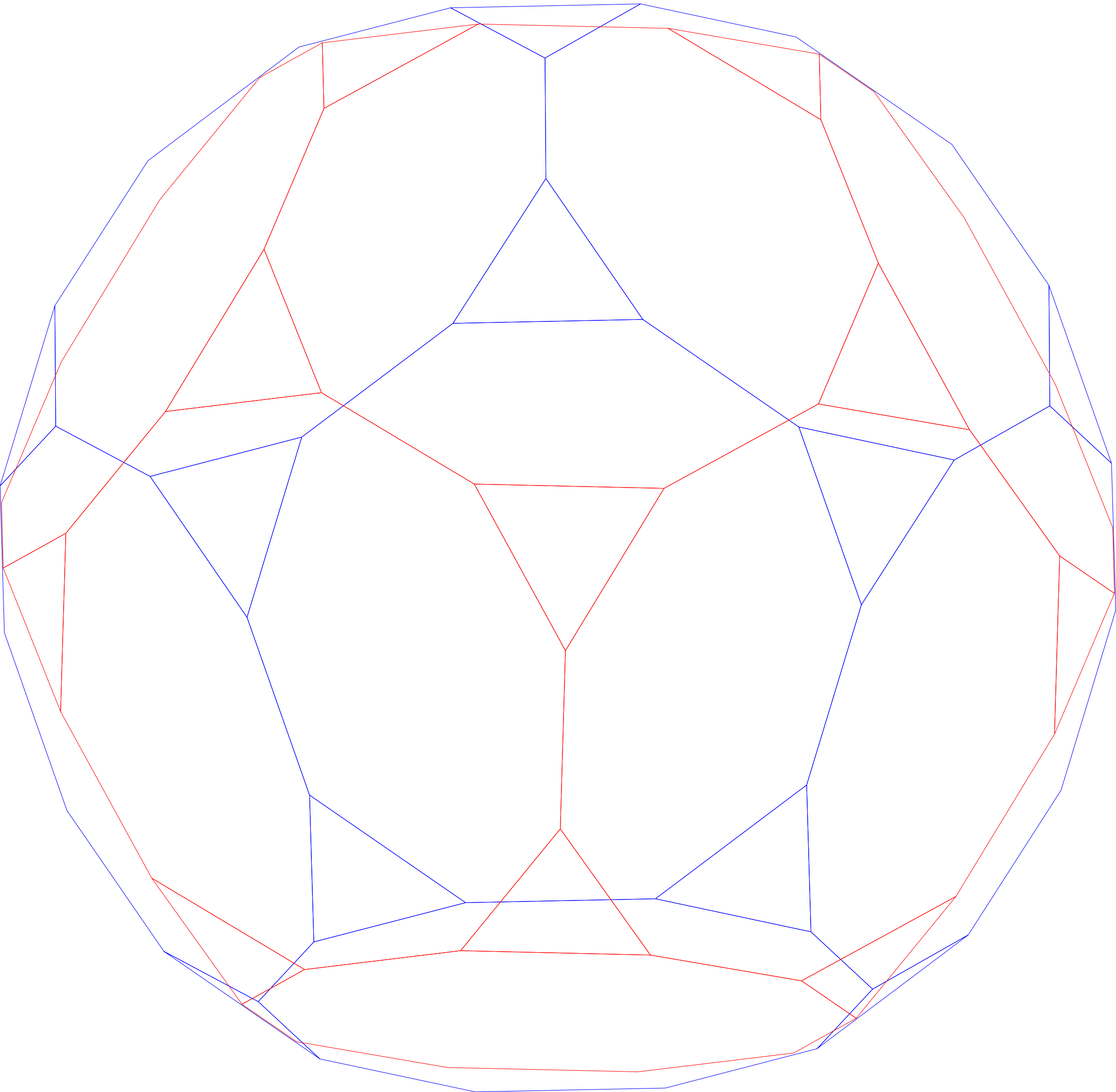
Truncated Dodecahedron
