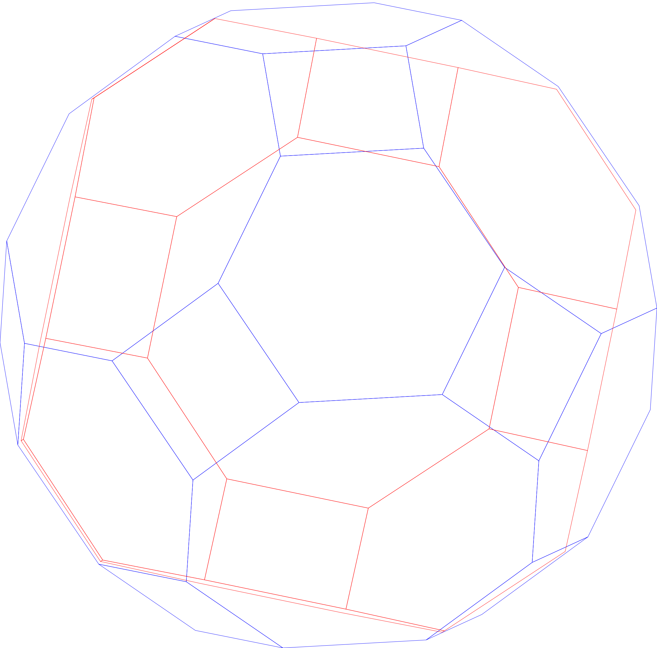
Truncated Cuboctahedron
