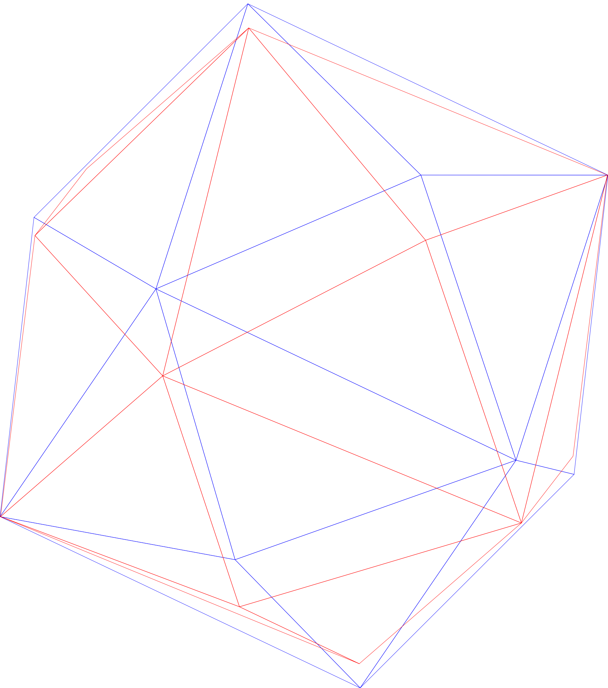
Tetrakis Hexahedron
