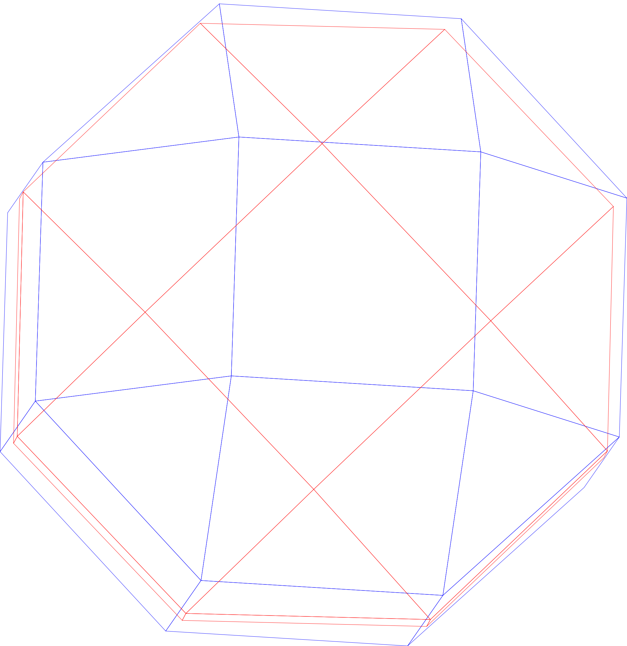
Rhombicuboctahedron
