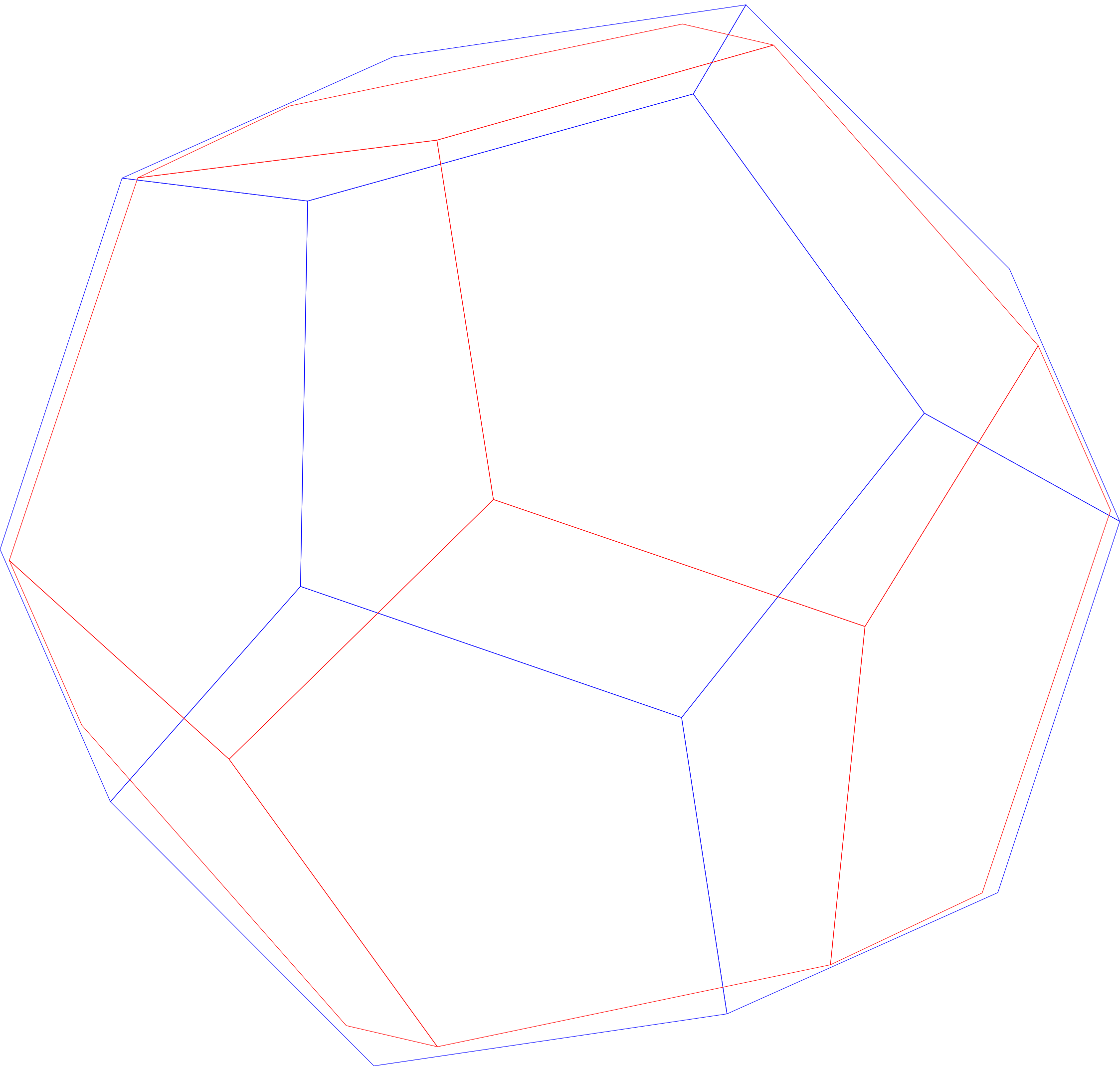
Dodecahedron
