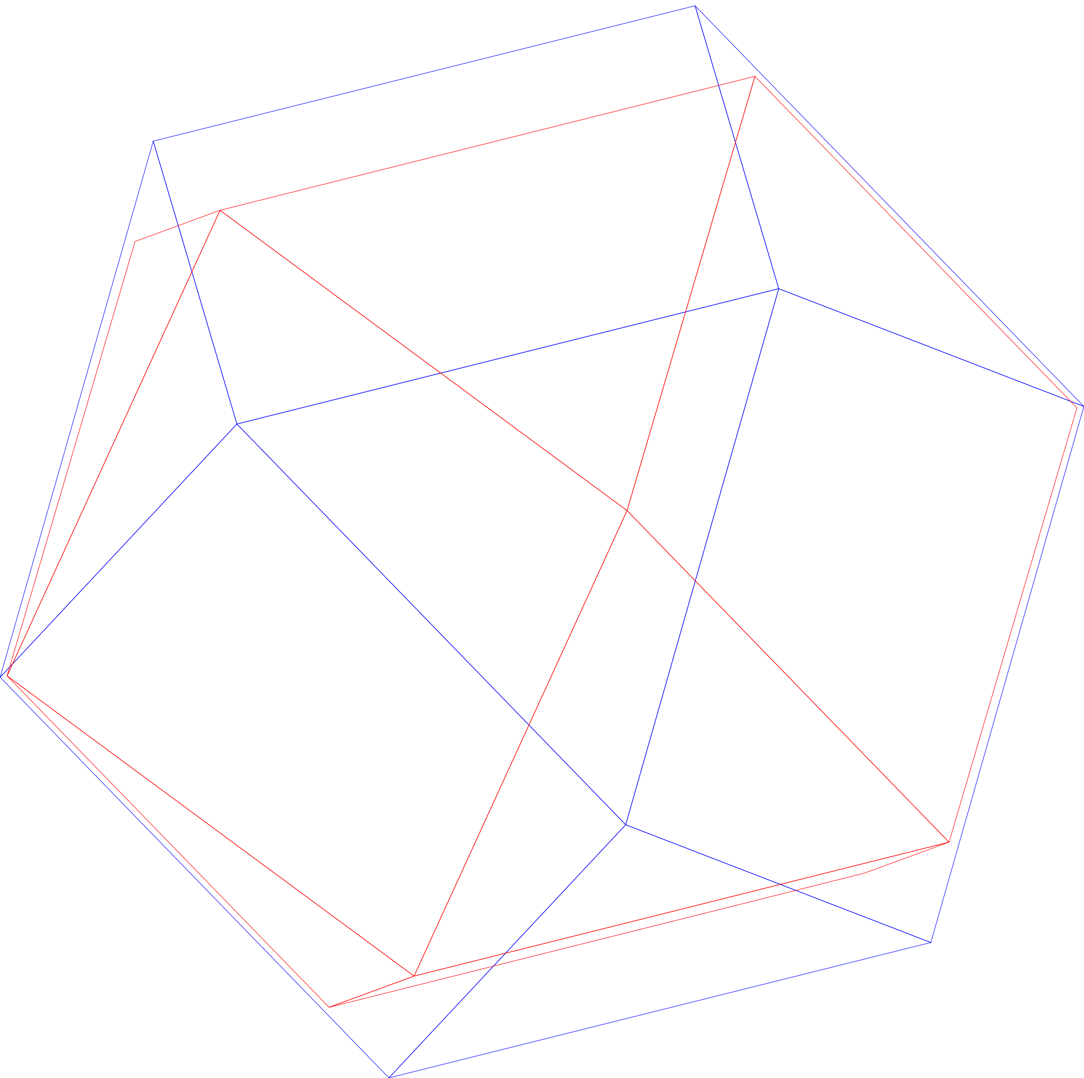
Cuboctahedron
